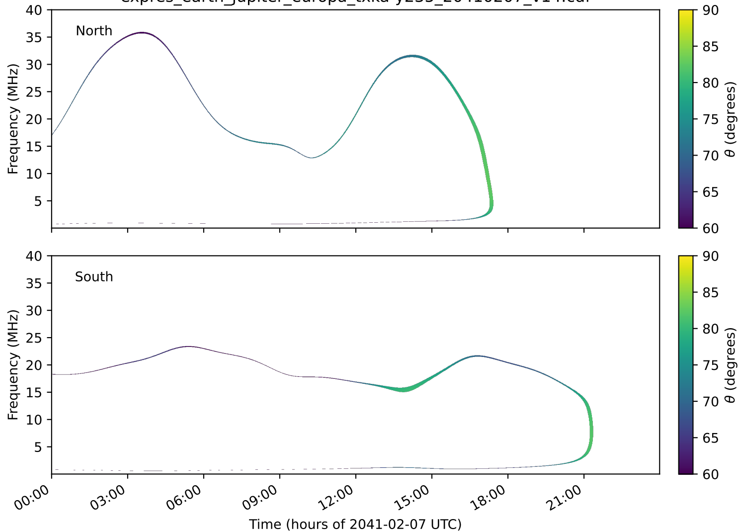
expres_earth_jupiter_europa_txka-y235_20410207_v14.cdf
