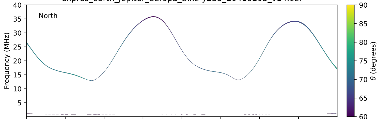
expres_earth_jupiter_europa_txka-y235_20410203_v14.cdf
