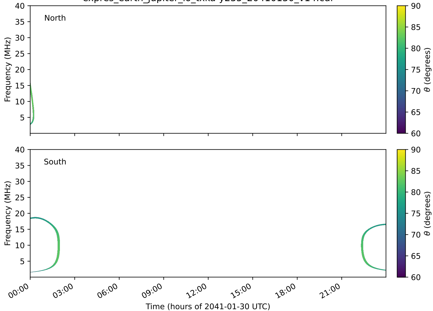
expres_earth_jupiter_io_txka-y235_20410130_v14.cdf
