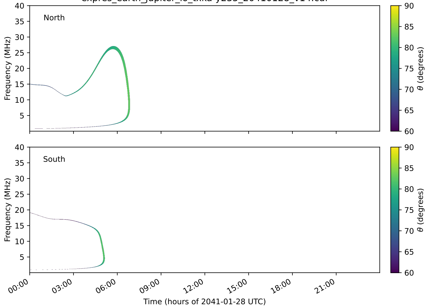
expres_earth_jupiter_io_txka-y235_20410128_v14.cdf
