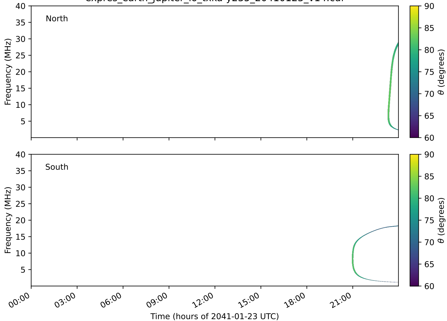
expres_earth_jupiter_io_txka-y235_20410123_v14.cdf
