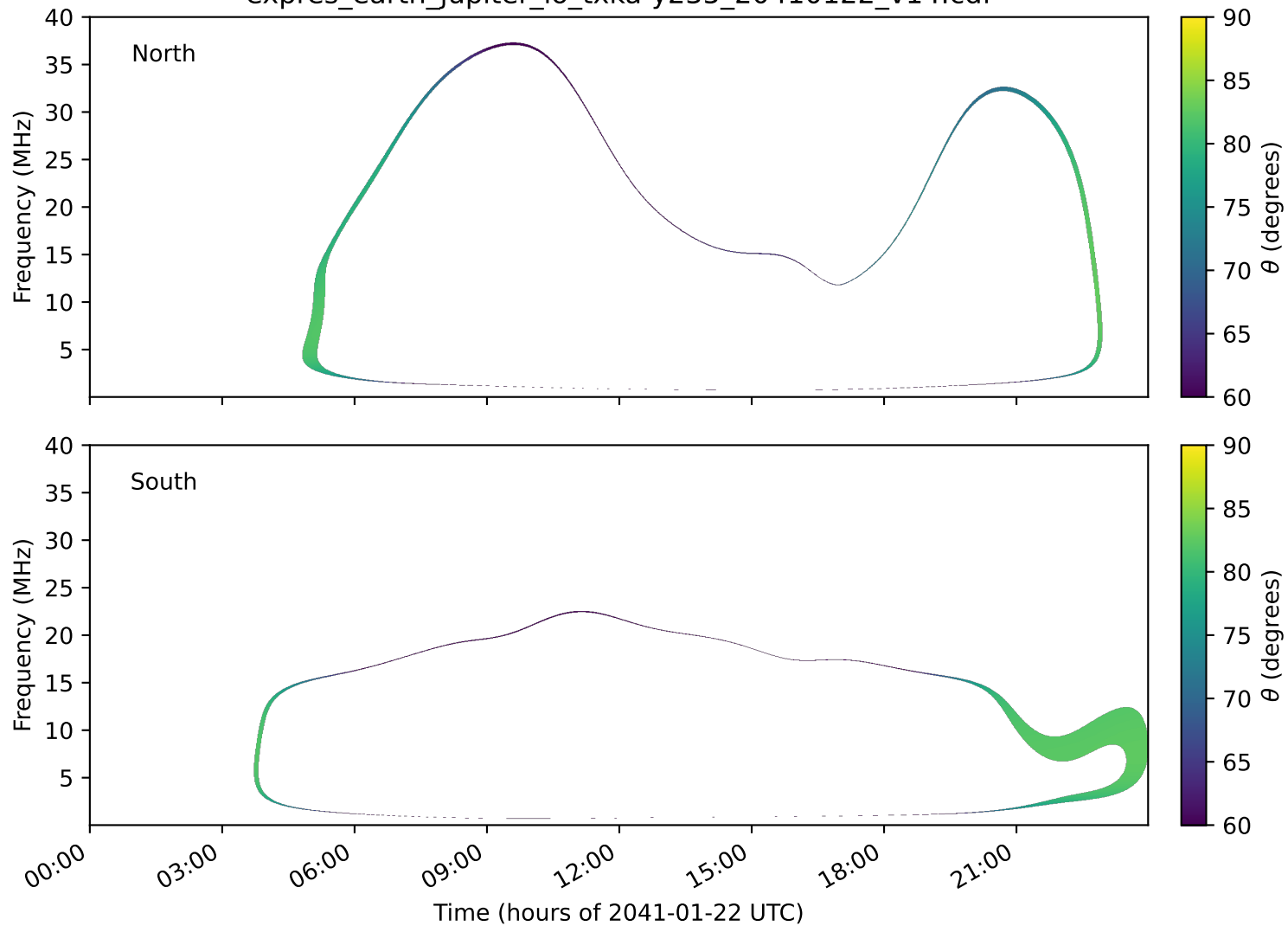
expres_earth_jupiter_io_txka-y235_20410122_v14.cdf
