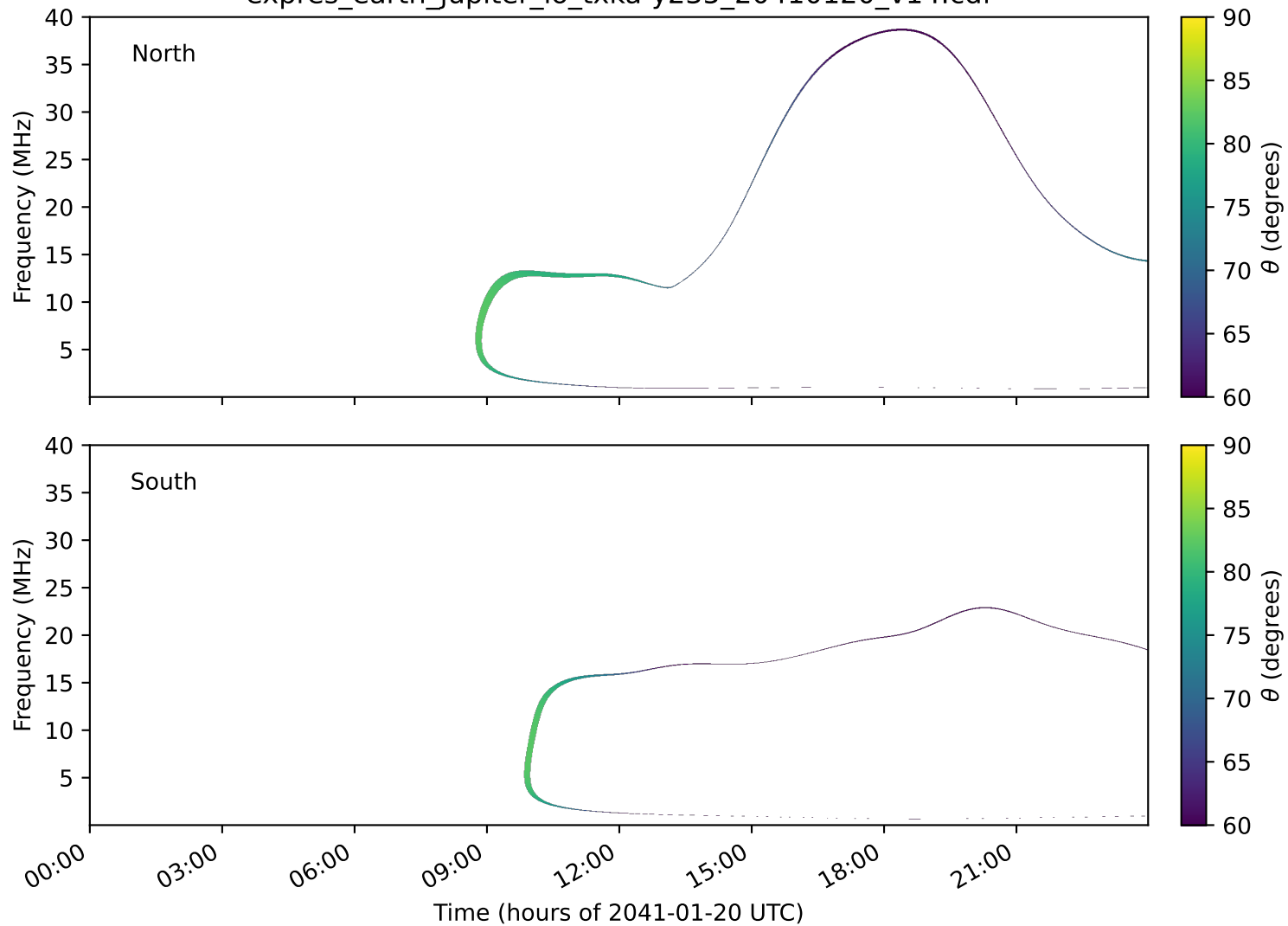
expres_earth_jupiter_io_txka-y235_20410120_v14.cdf
