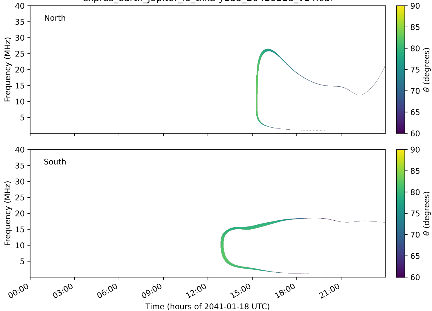
expres_earth_jupiter_io_txka-y235_20410118_v14.cdf
