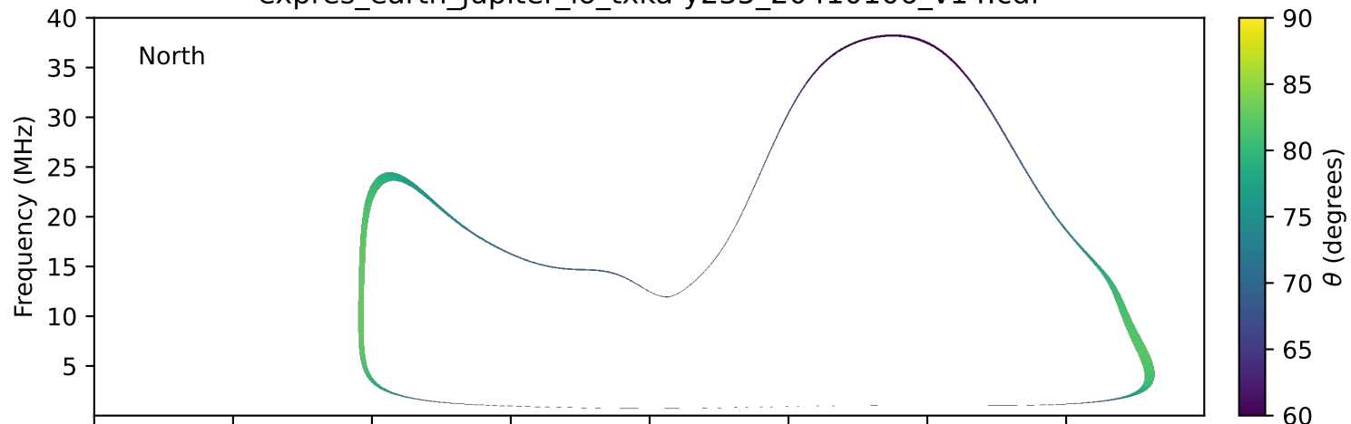
expres_earth_jupiter_io_txka-y235_20410106_v14.cdf
