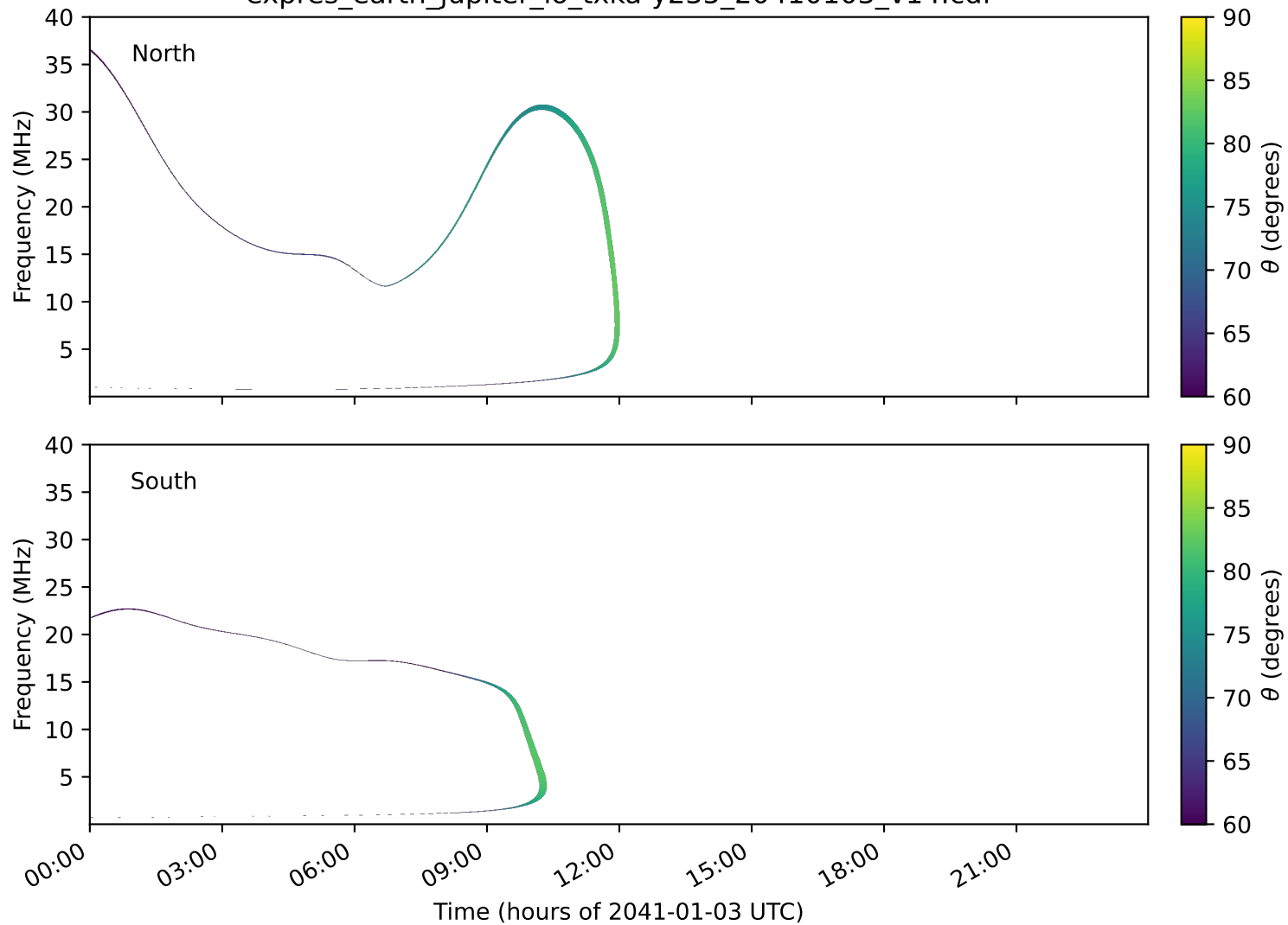
expres_earth_jupiter_io_txka-y235_20410103_v14.cdf
