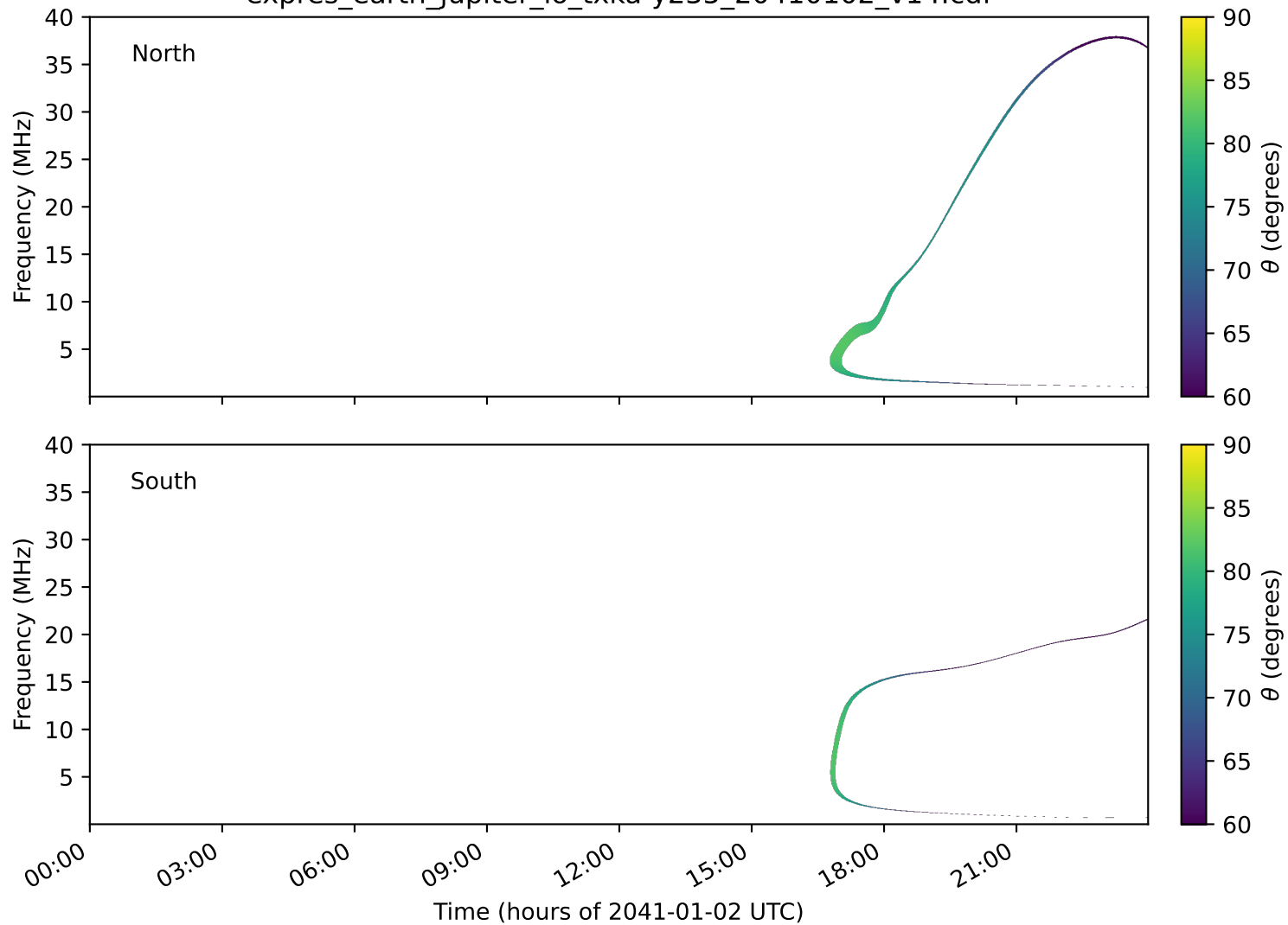
expres_earth_jupiter_io_txka-y235_20410102_v14.cdf
