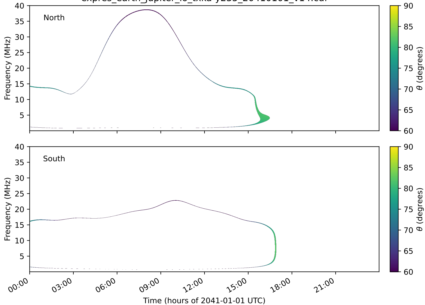
expres_earth_jupiter_io_txka-y235_20410101_v14.cdf
