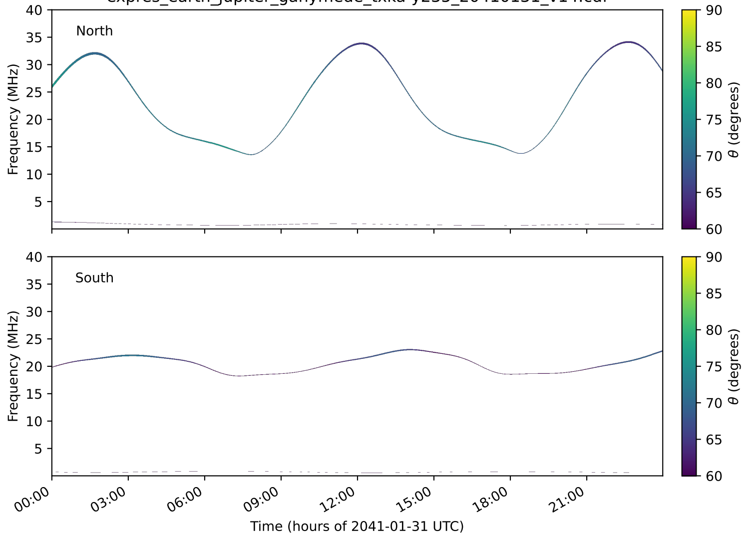
expres_earth_jupiter_ganymede_txka-y235_20410131_v14.cdf
