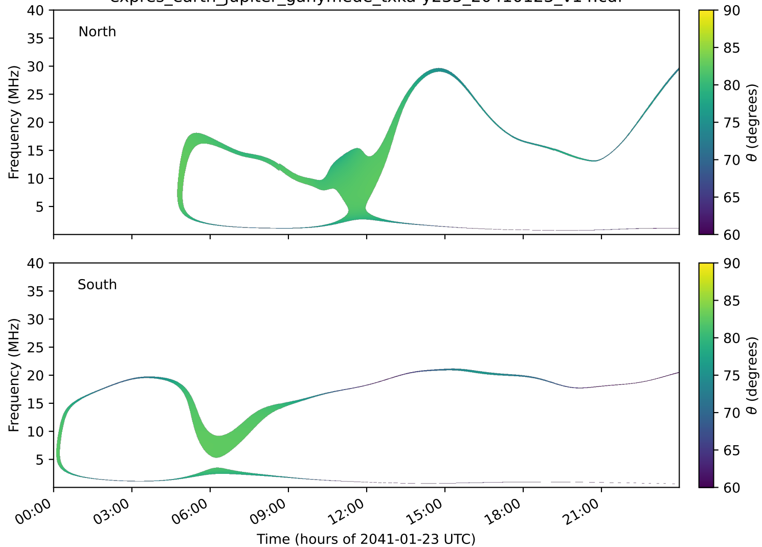
expres_earth_jupiter_ganymede_txka-y235_20410123_v14.cdf
