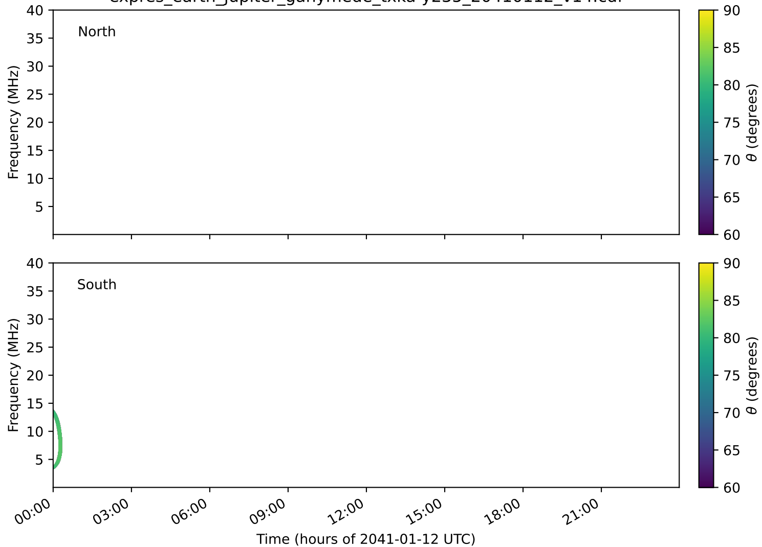
expres_earth_jupiter_ganymede_txka-y235_20410112_v14.cdf
