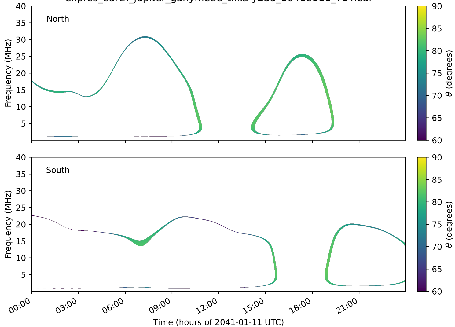
expres_earth_jupiter_ganymede_txka-y235_20410111_v14.cdf
