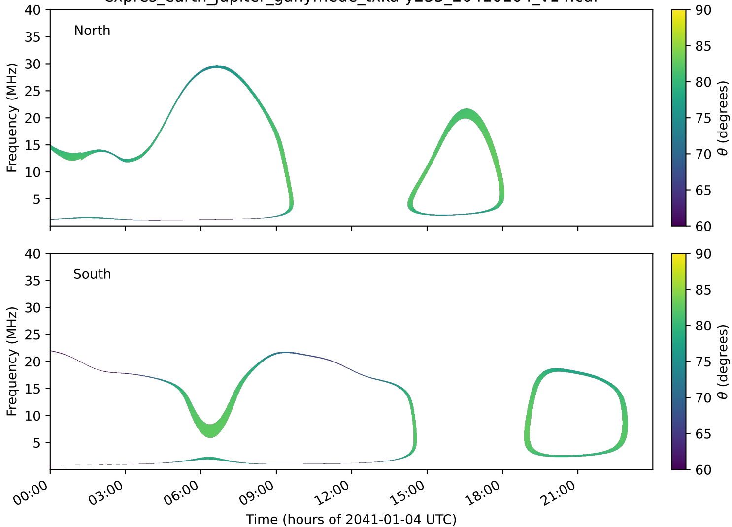
expres_earth_jupiter_ganymede_txka-y235_20410104_v14.cdf
