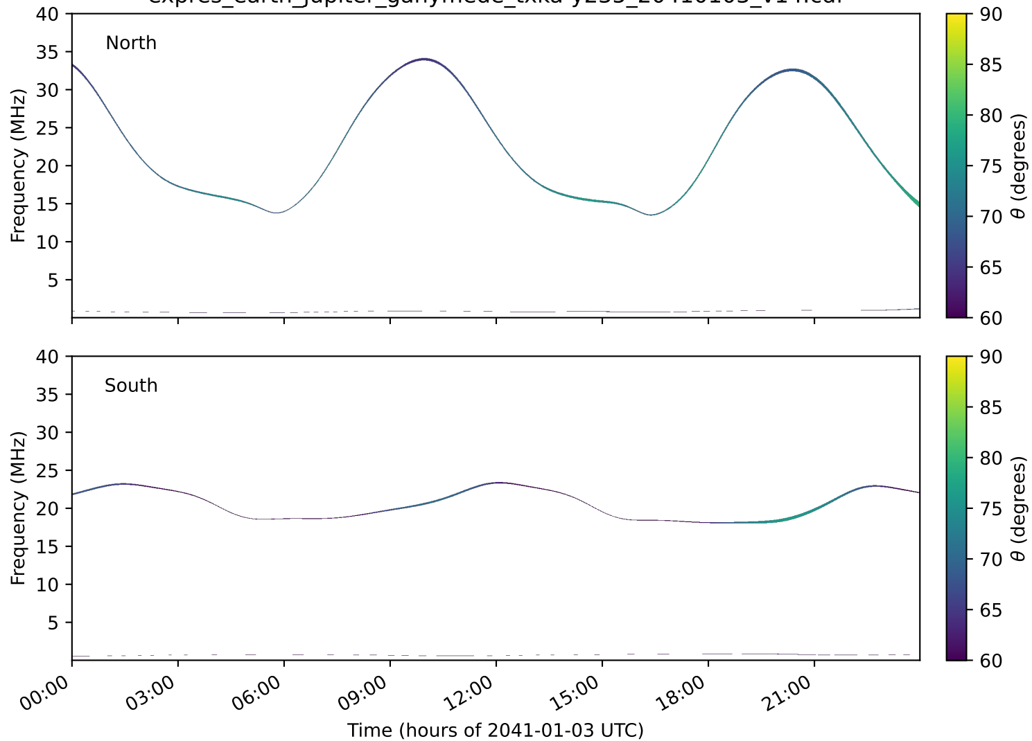
expres_earth_jupiter_ganymede_txka-y235_20410103_v14.cdf
