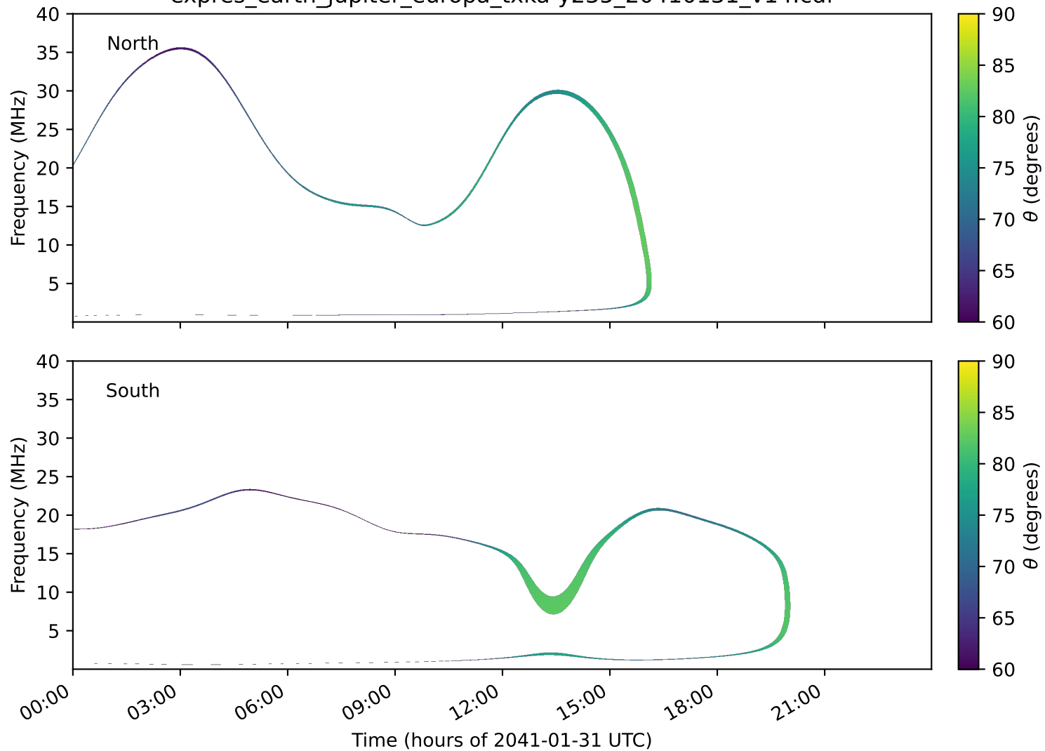
expres_earth_jupiter_europa_txka-y235_20410131_v14.cdf
