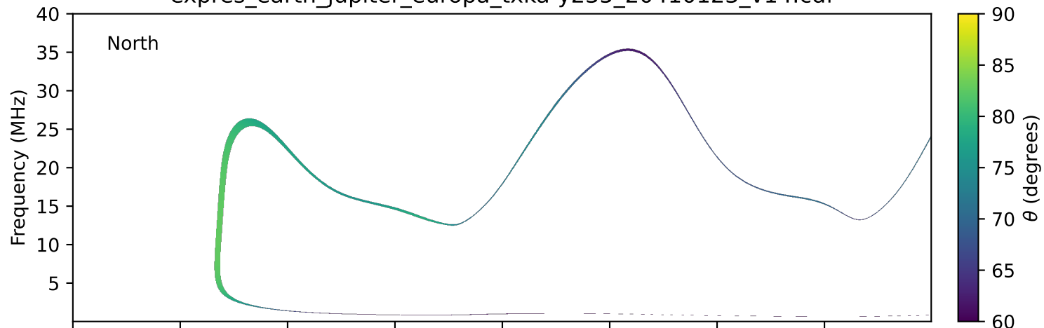
expres_earth_jupiter_europa_txka-y235_20410123_v14.cdf
