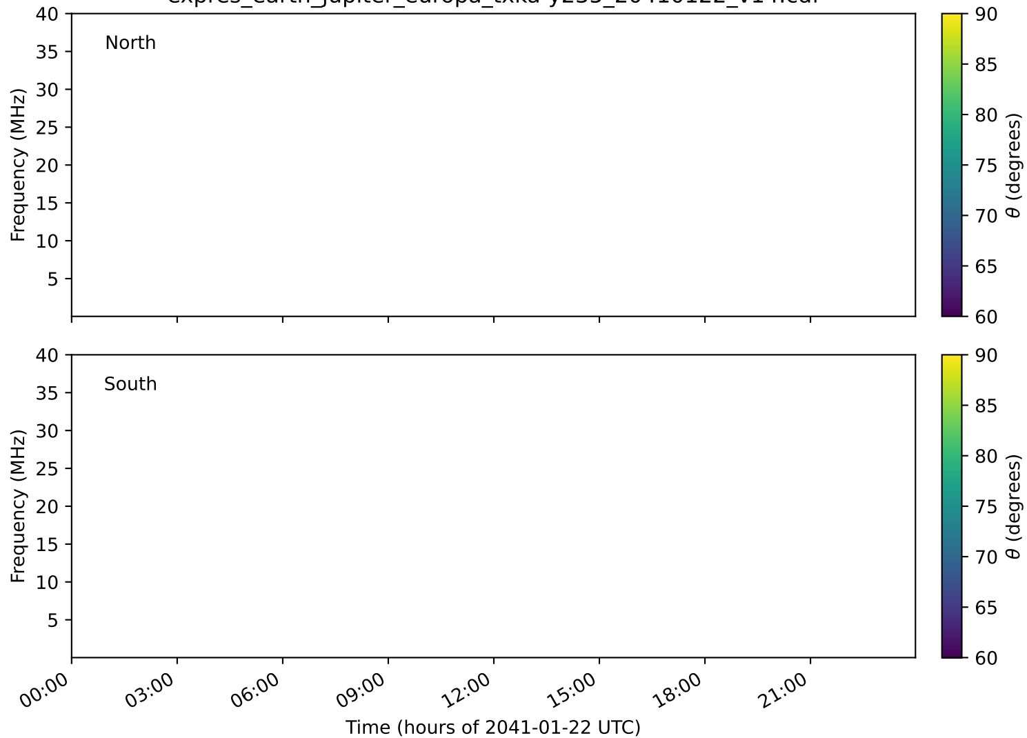
expres_earth_jupiter_europa_txka-y235_20410122_v14.cdf
