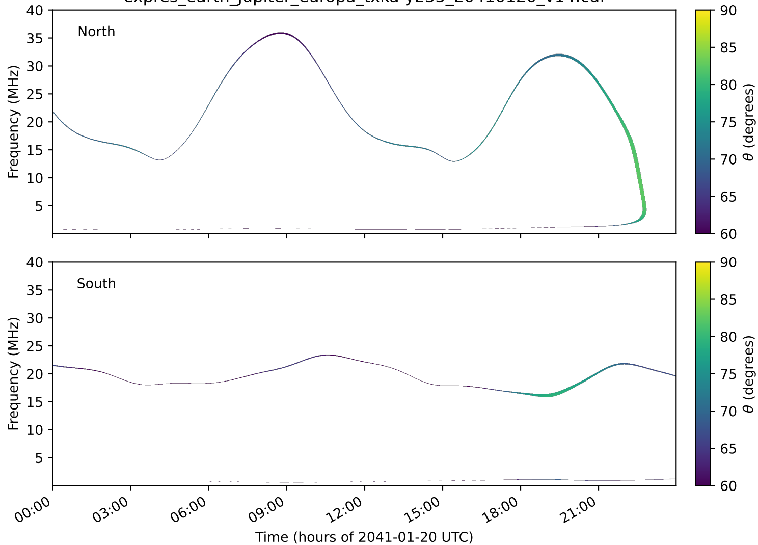
expres_earth_jupiter_europa_txka-y235_20410120_v14.cdf
