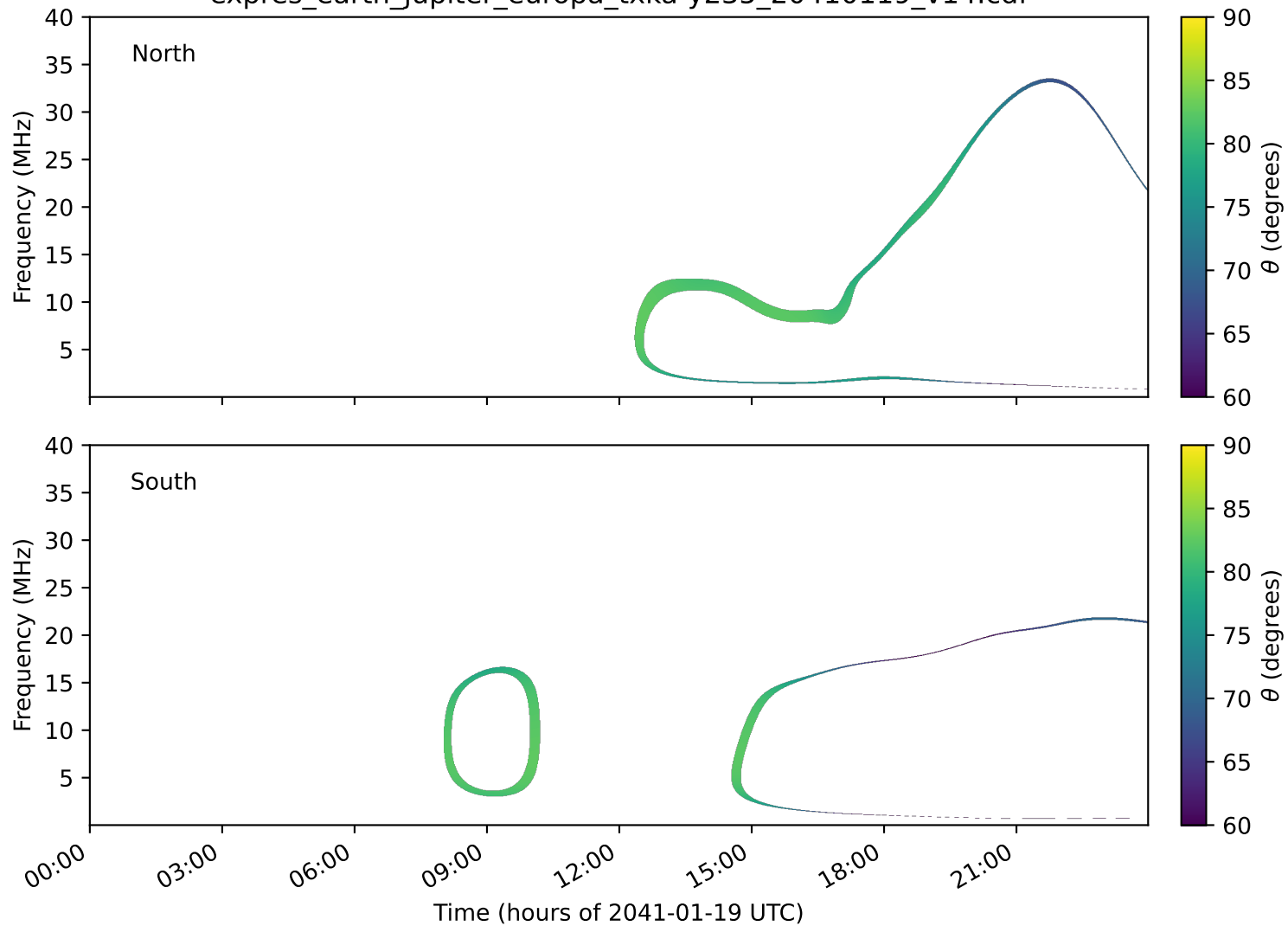
expres_earth_jupiter_europa_txka-y235_20410119_v14.cdf
