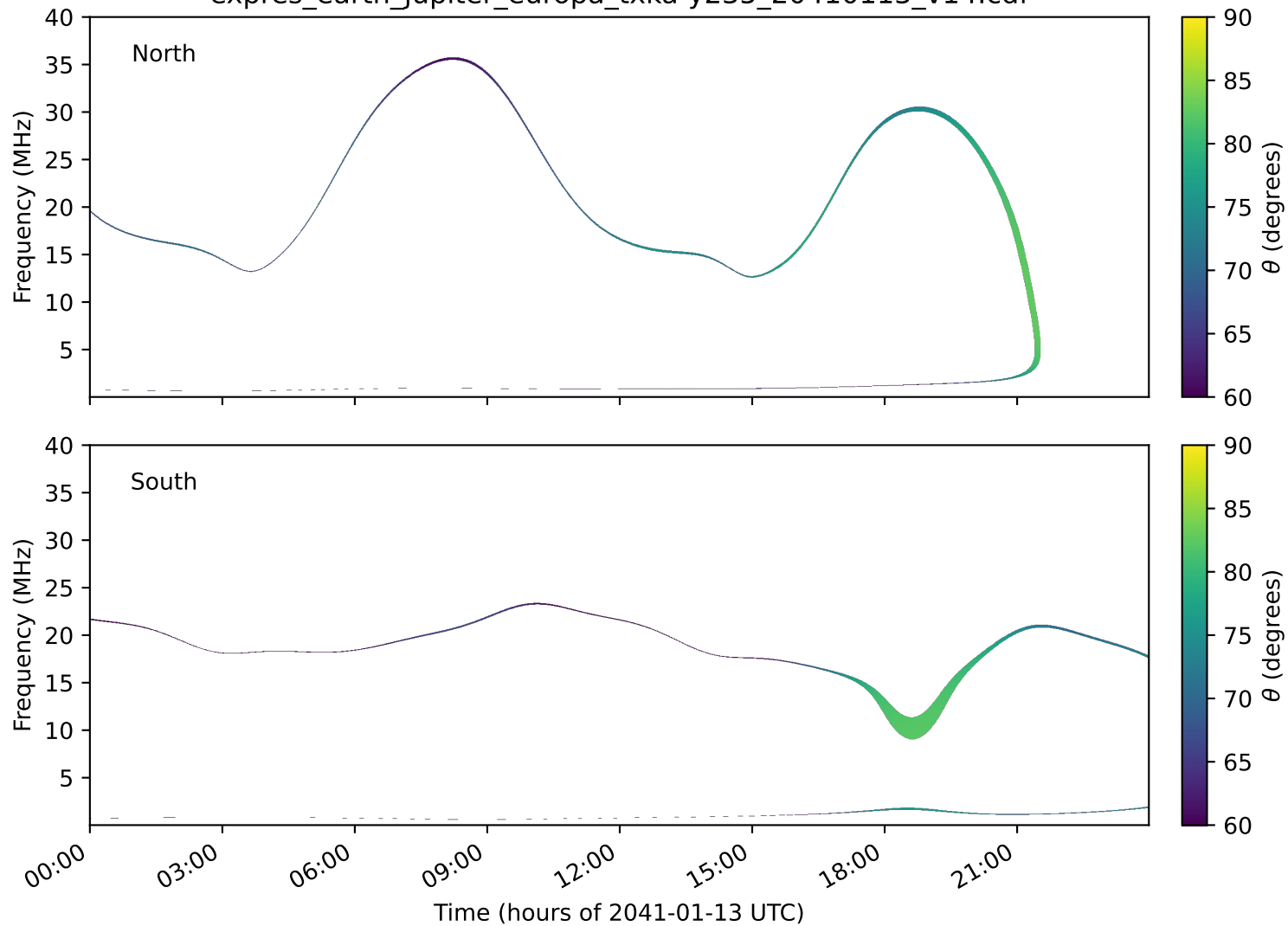
expres_earth_jupiter_europa_txka-y235_20410113_v14.cdf
