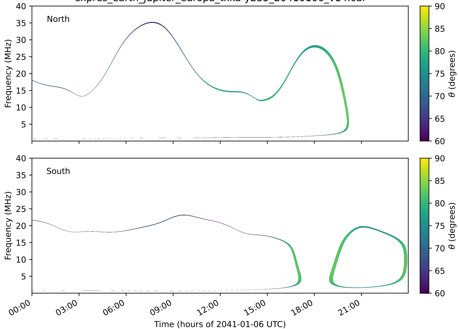
expres_earth_jupiter_europa_txka-y235_20410106_v14.cdf
