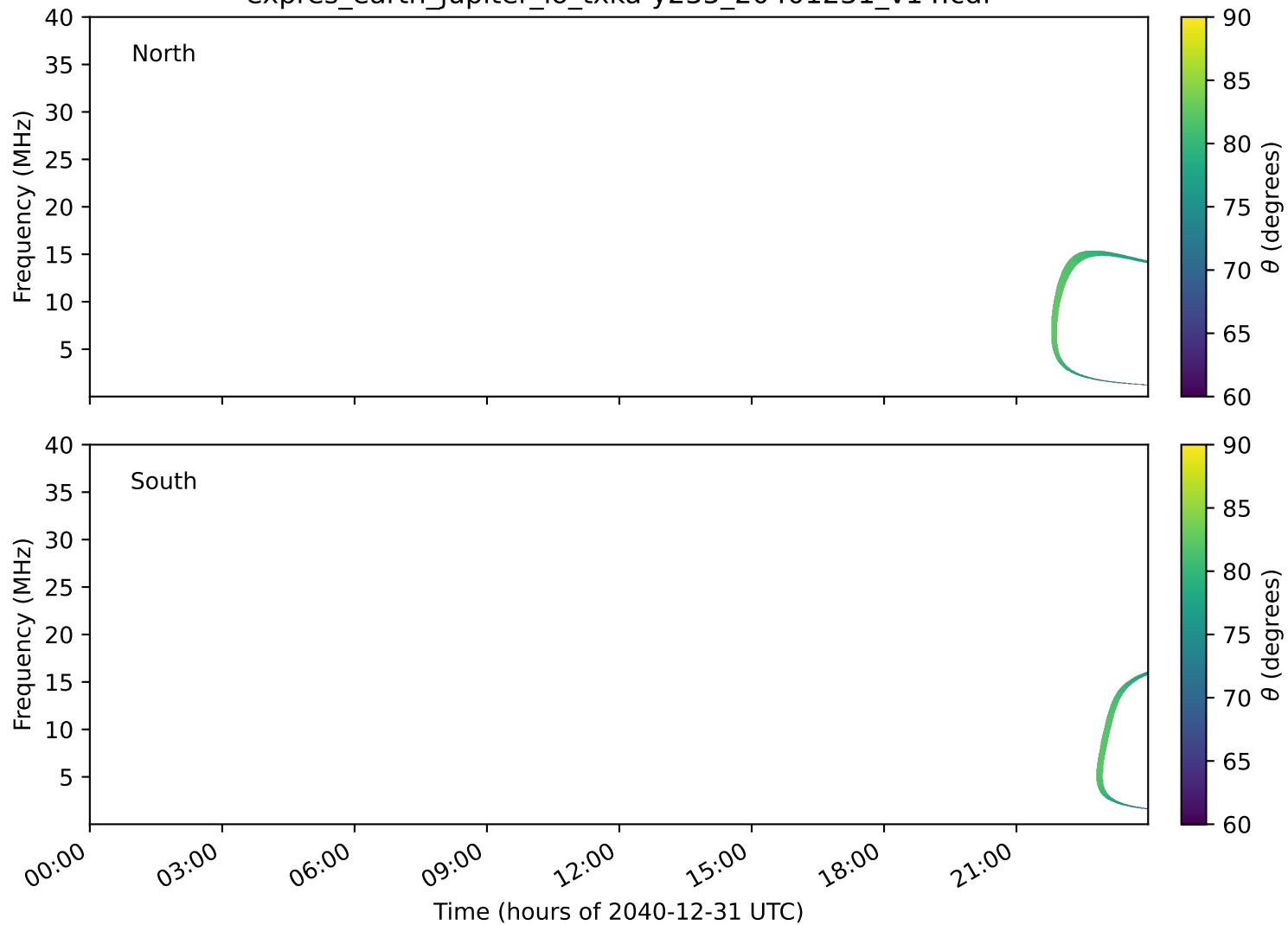
expres_earth_jupiter_io_txka-y235_20401231_v14.cdf
