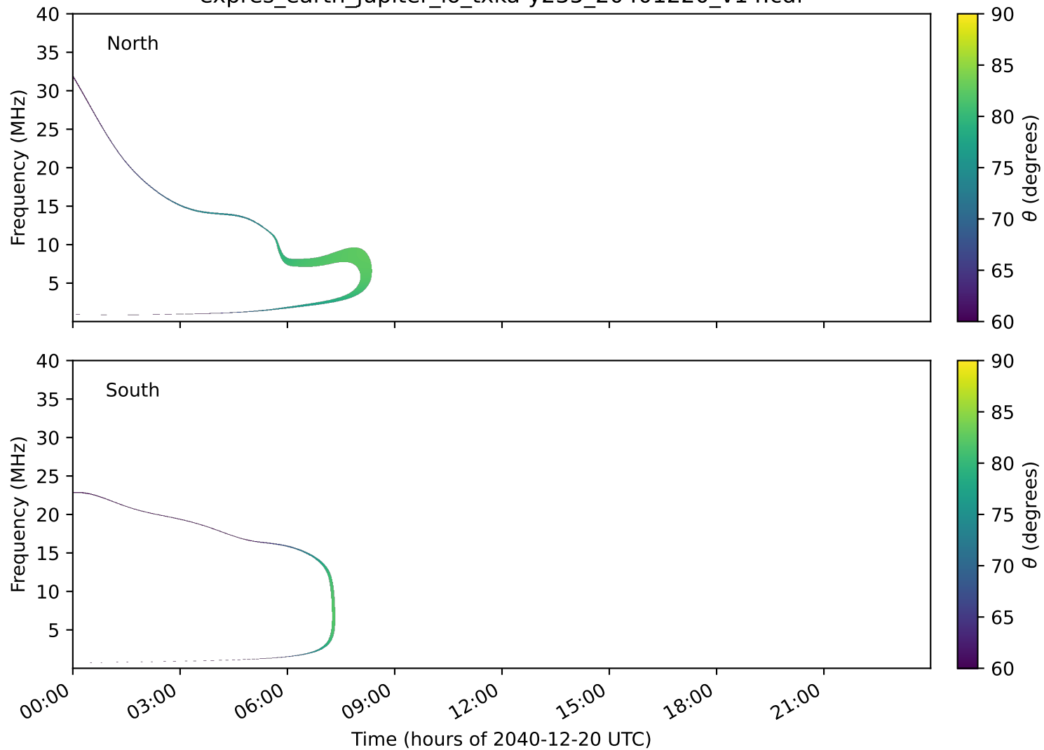
expres_earth_jupiter_io_txka-y235_20401220_v14.cdf
