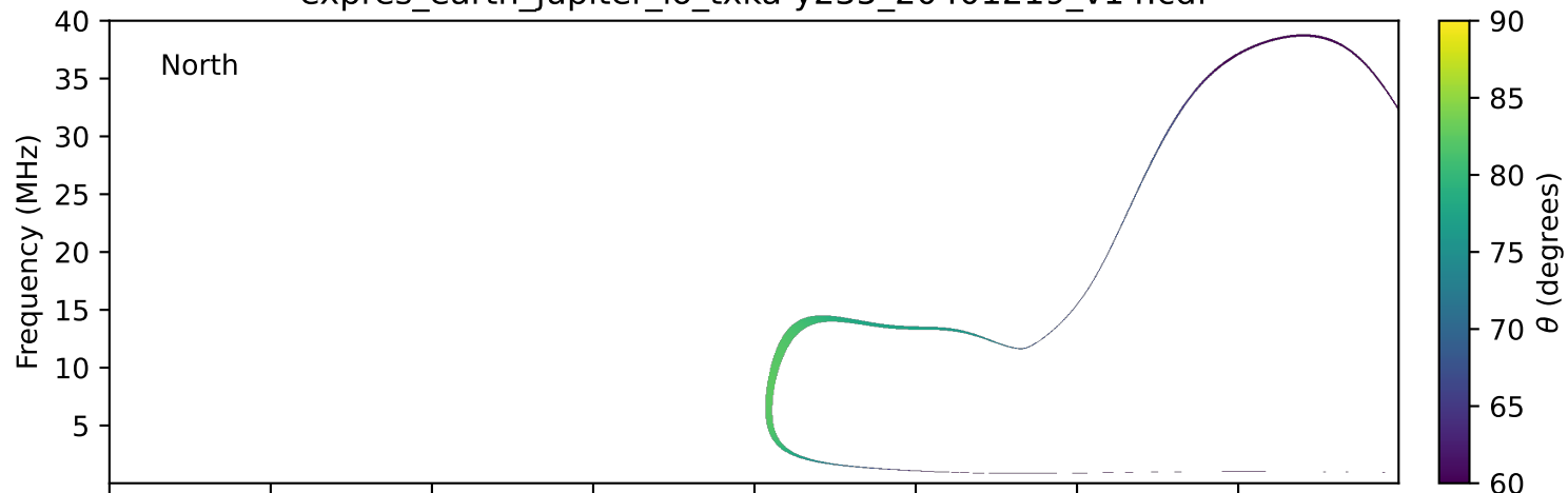
expres_earth_jupiter_io_txka-y235_20401219_v14.cdf
