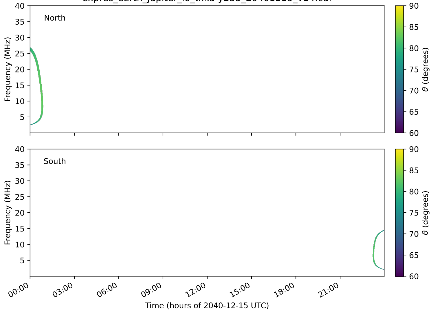
expres_earth_jupiter_io_txka-y235_20401215_v14.cdf
