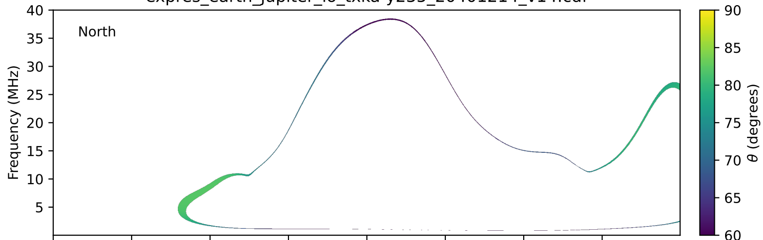
expres_earth_jupiter_io_txka-y235_20401214_v14.cdf
