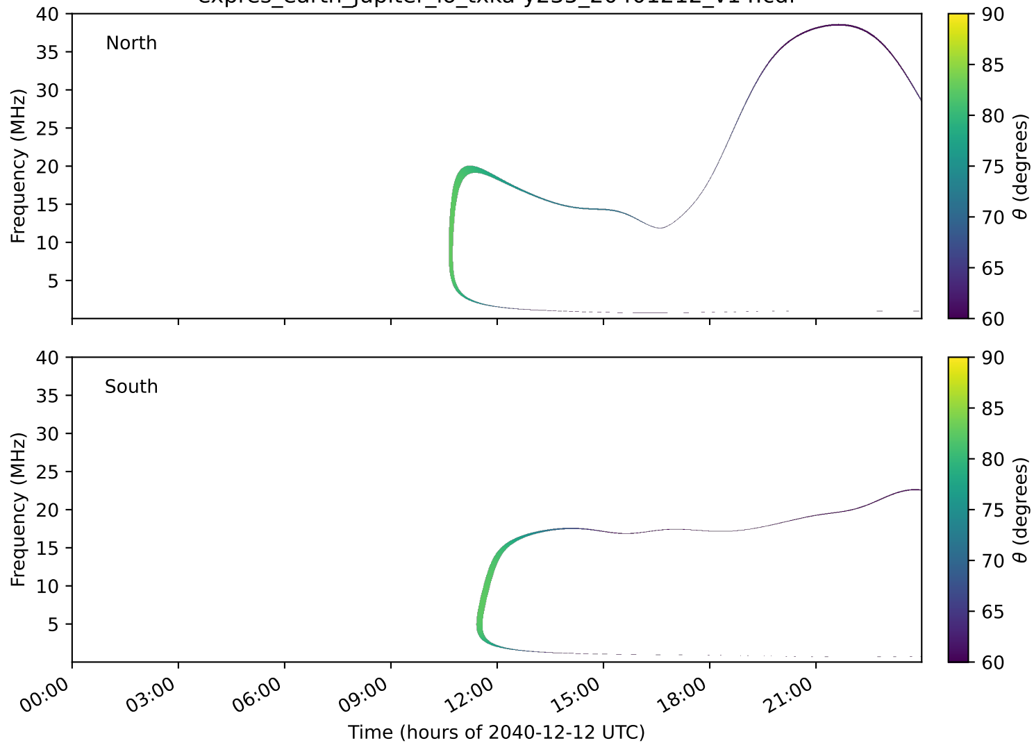
expres_earth_jupiter_io_txka-y235_20401212_v14.cdf
