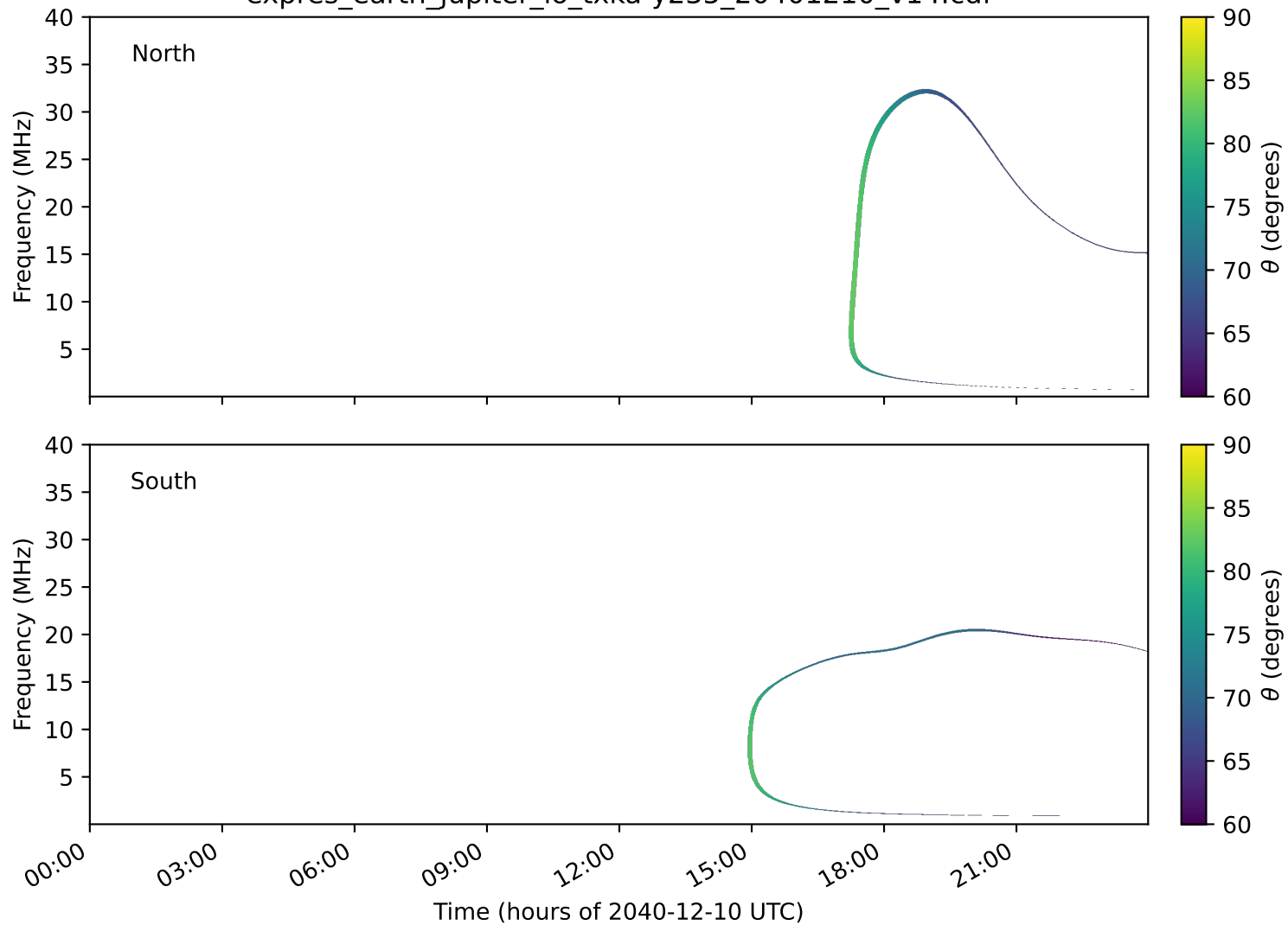
expres_earth_jupiter_io_txka-y235_20401210_v14.cdf
