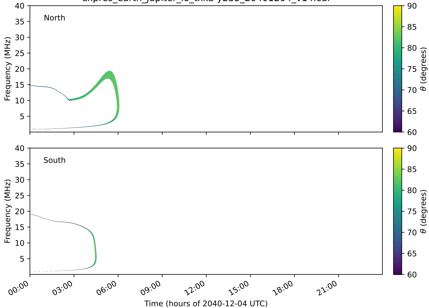
expres_earth_jupiter_io_txka-y235_20401204_v14.cdf
