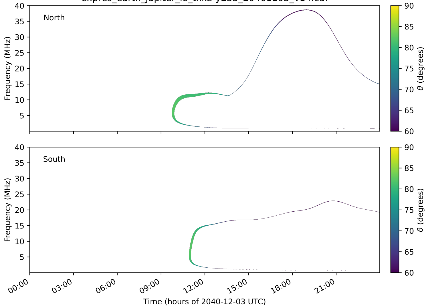
expres_earth_jupiter_io_txka-y235_20401203_v14.cdf
