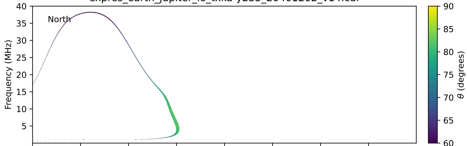
expres_earth_jupiter_io_txka-y235_20401202_v14.cdf
