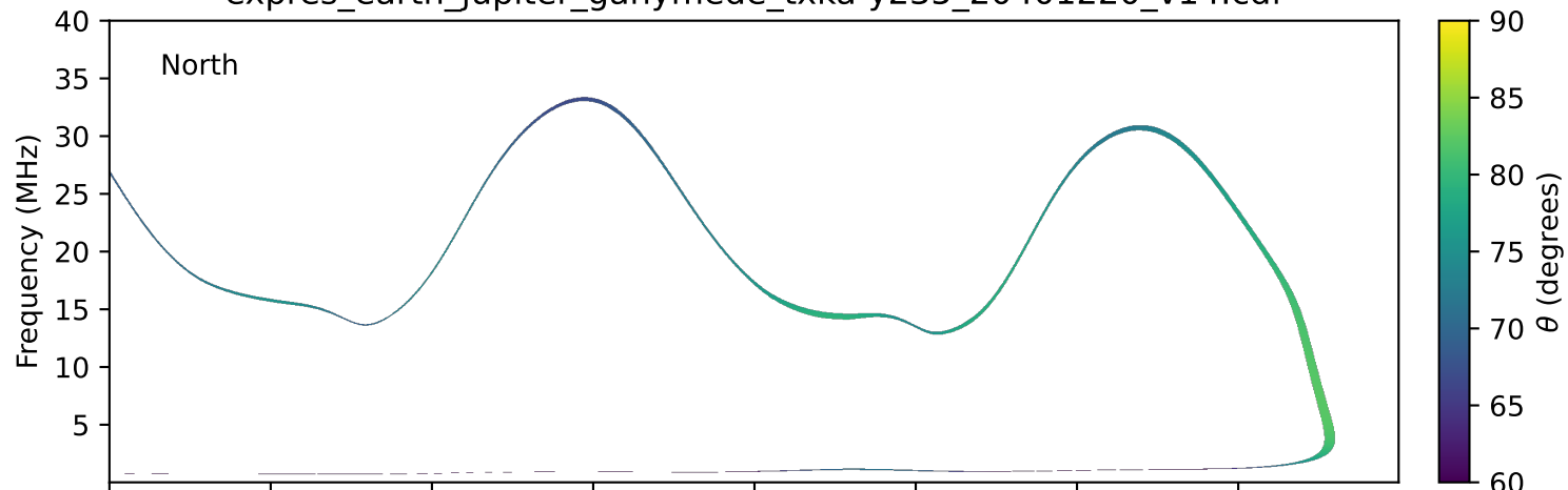
expres_earth_jupiter_ganymede_txka-y235_20401220_v14.cdf
