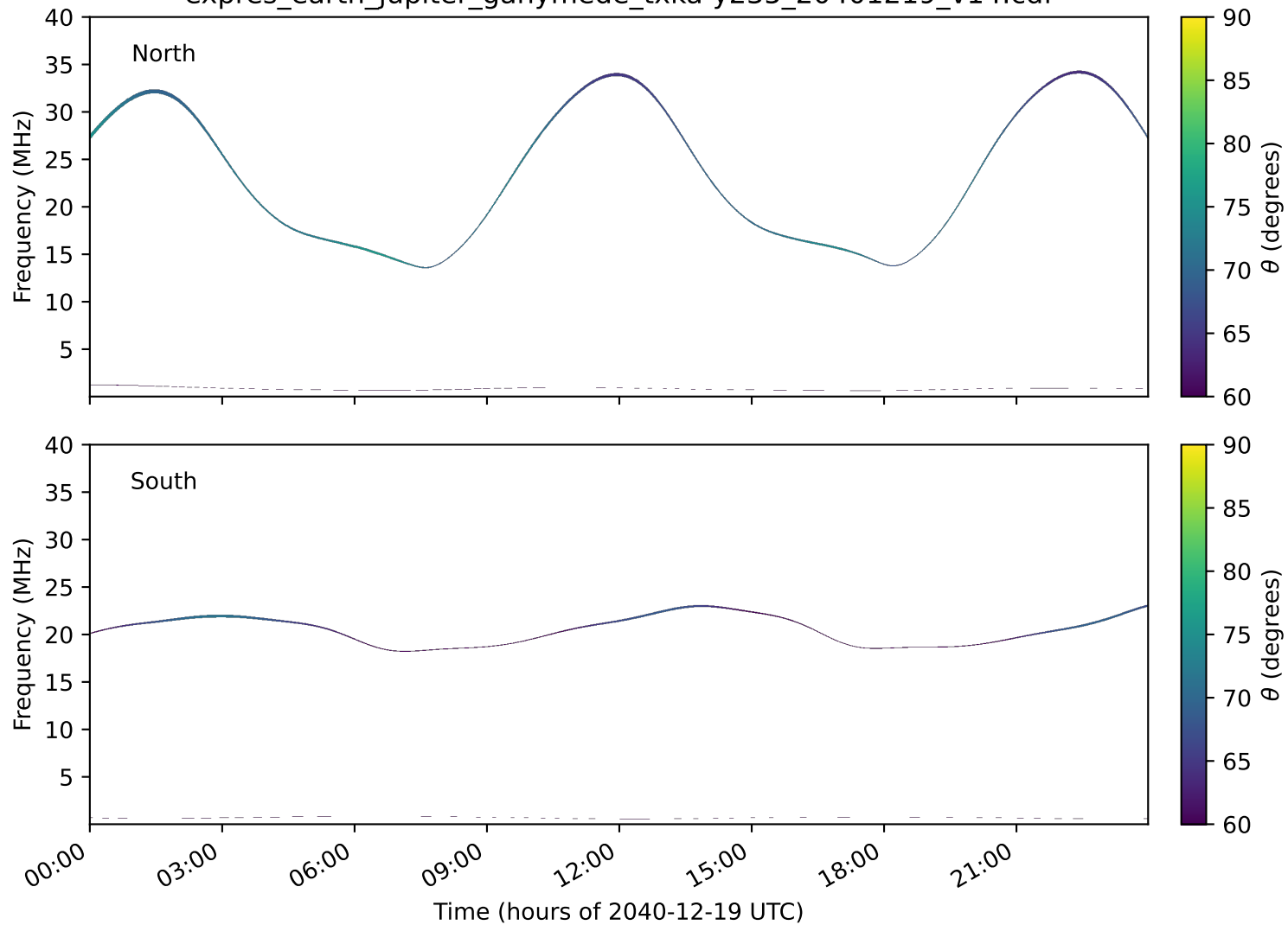
expres_earth_jupiter_ganymede_txka-y235_20401219_v14.cdf
