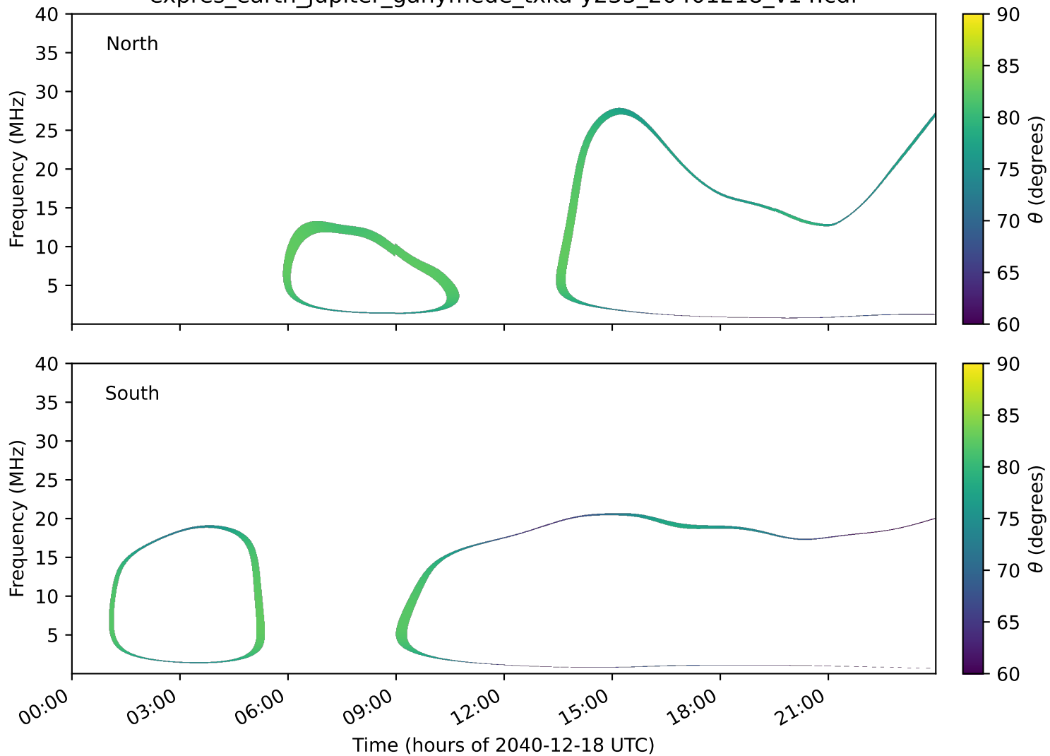
expres_earth_jupiter_ganymede_txka-y235_20401218_v14.cdf
