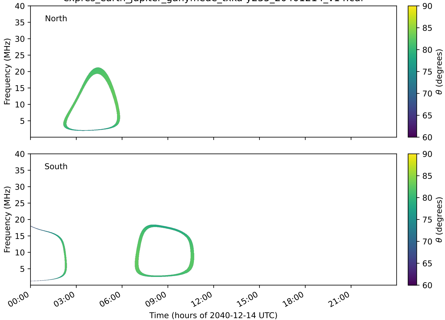
expres_earth_jupiter_ganymede_txka-y235_20401214_v14.cdf
