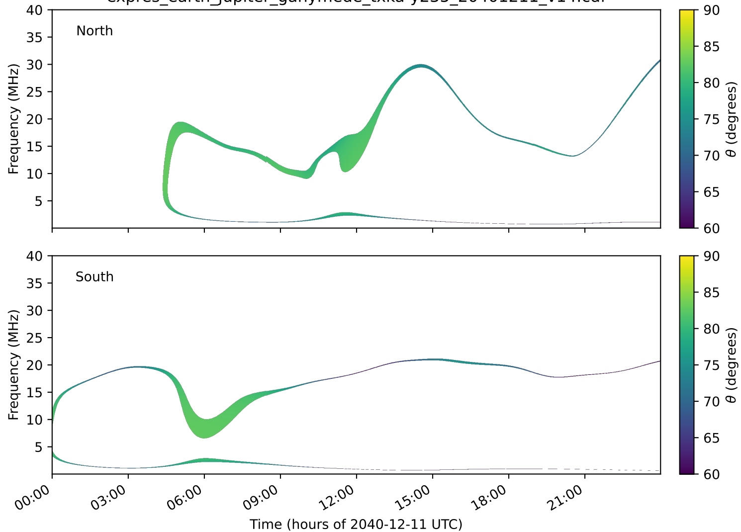
expres_earth_jupiter_ganymede_txka-y235_20401211_v14.cdf
