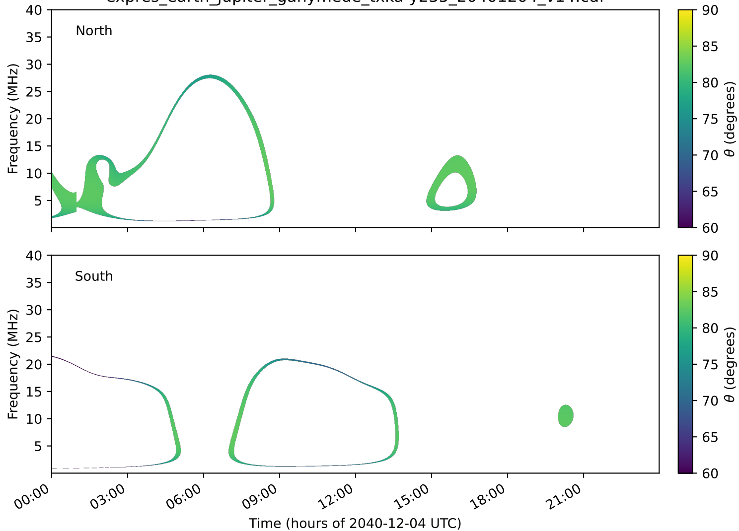
expres_earth_jupiter_ganymede_txka-y235_20401204_v14.cdf
