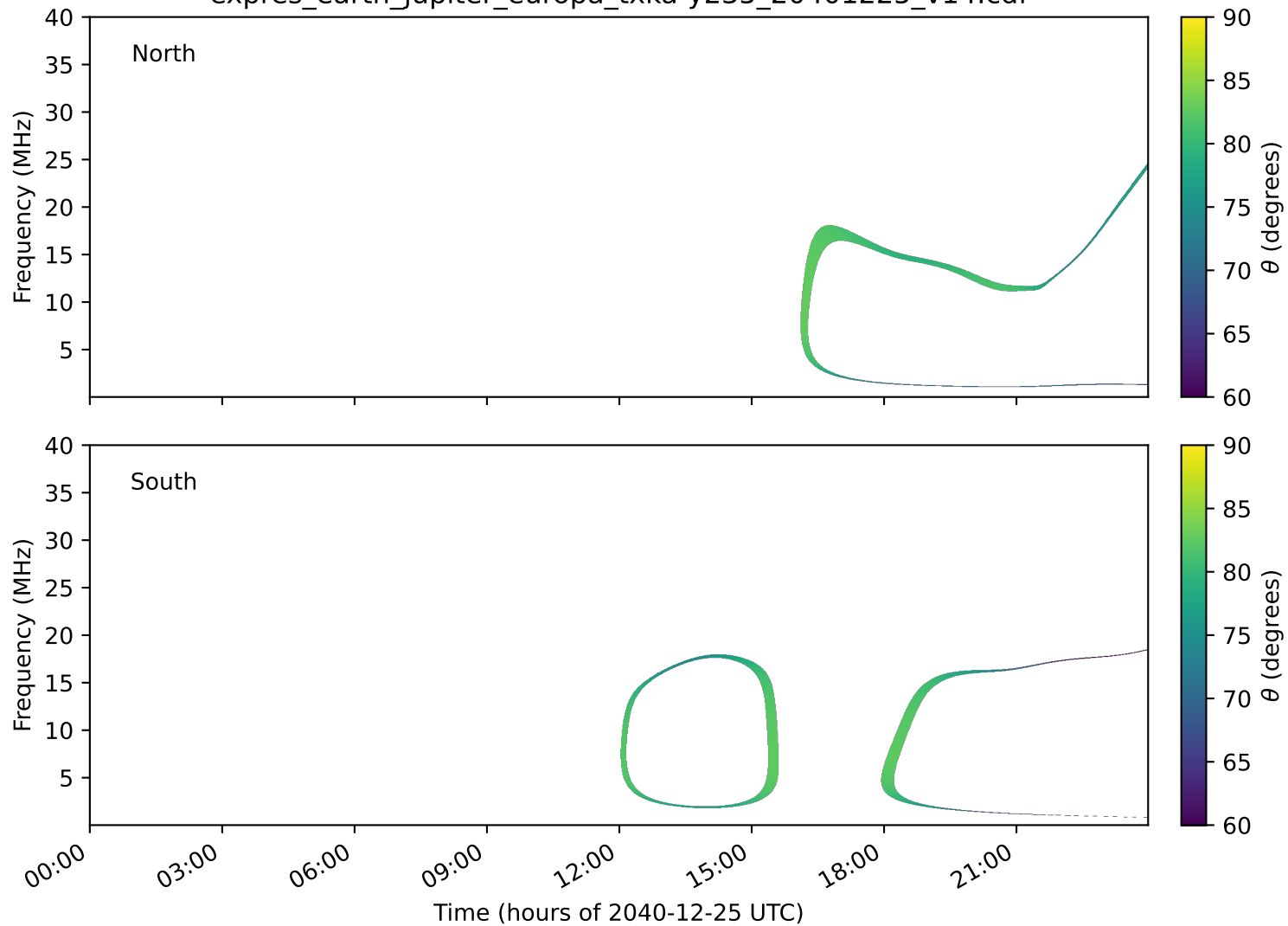
expres_earth_jupiter_europa_txka-y235_20401225_v14.cdf
