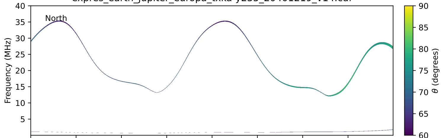
expres_earth_jupiter_europa_txka-y235_20401219_v14.cdf
