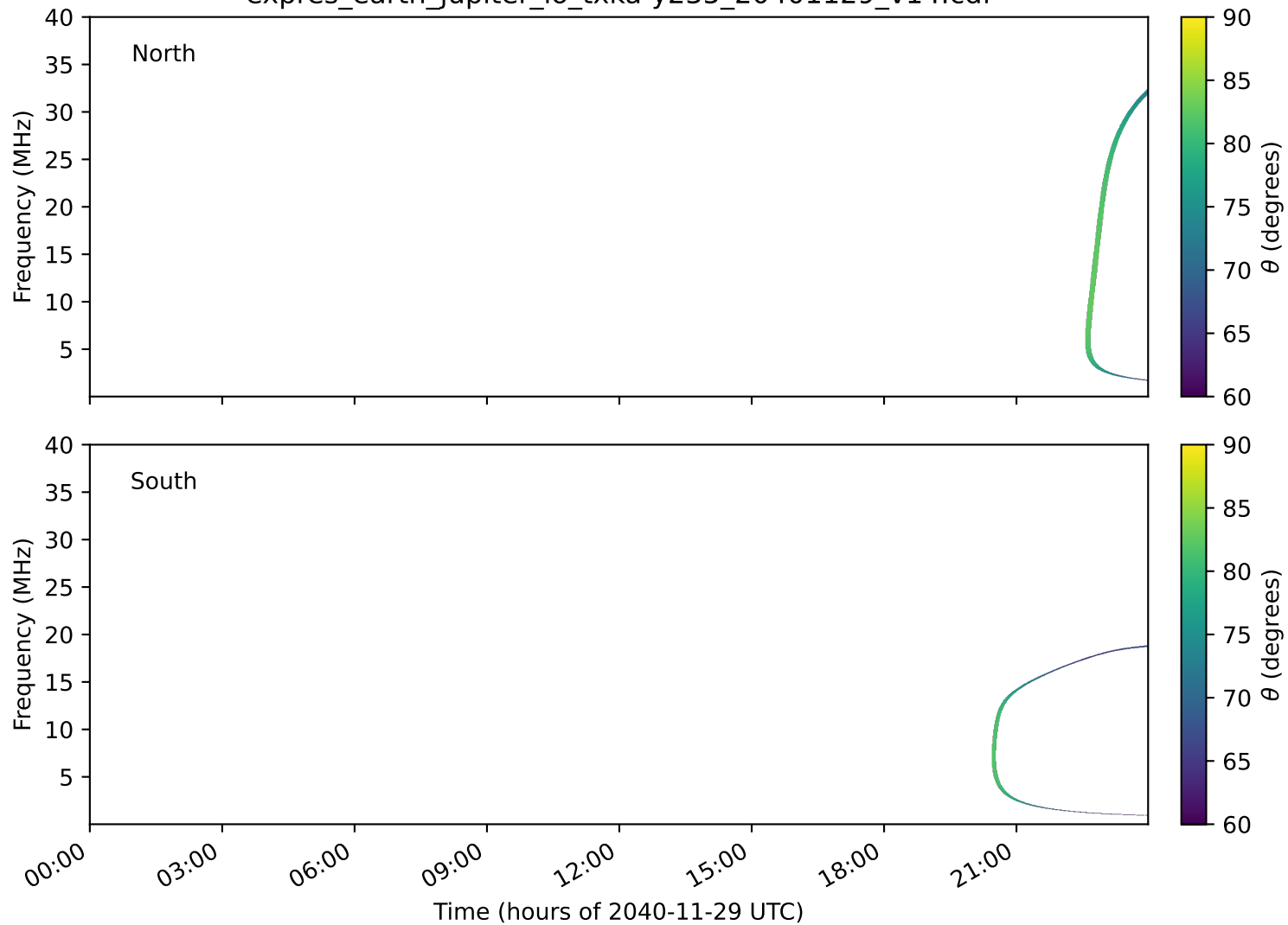
expres_earth_jupiter_io_txka-y235_20401129_v14.cdf
