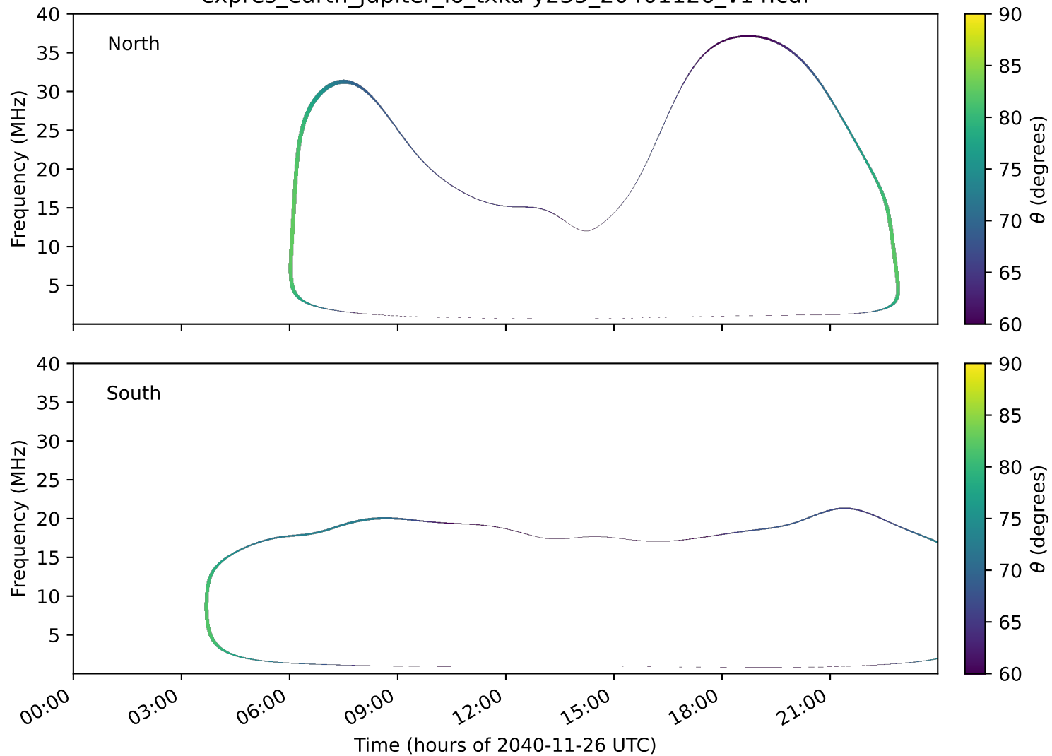
expres_earth_jupiter_io_txka-y235_20401126_v14.cdf
