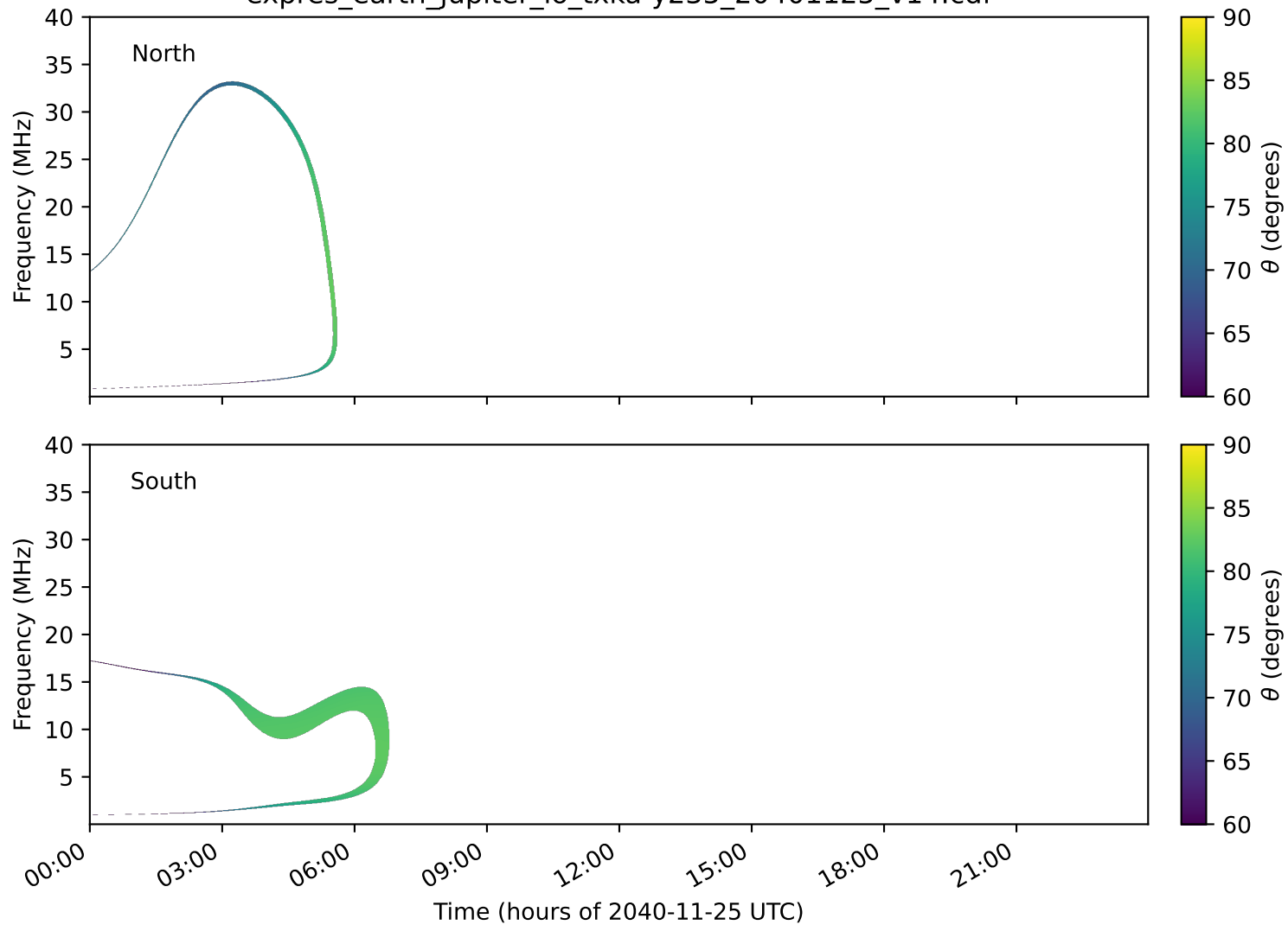
expres_earth_jupiter_io_txka-y235_20401125_v14.cdf
