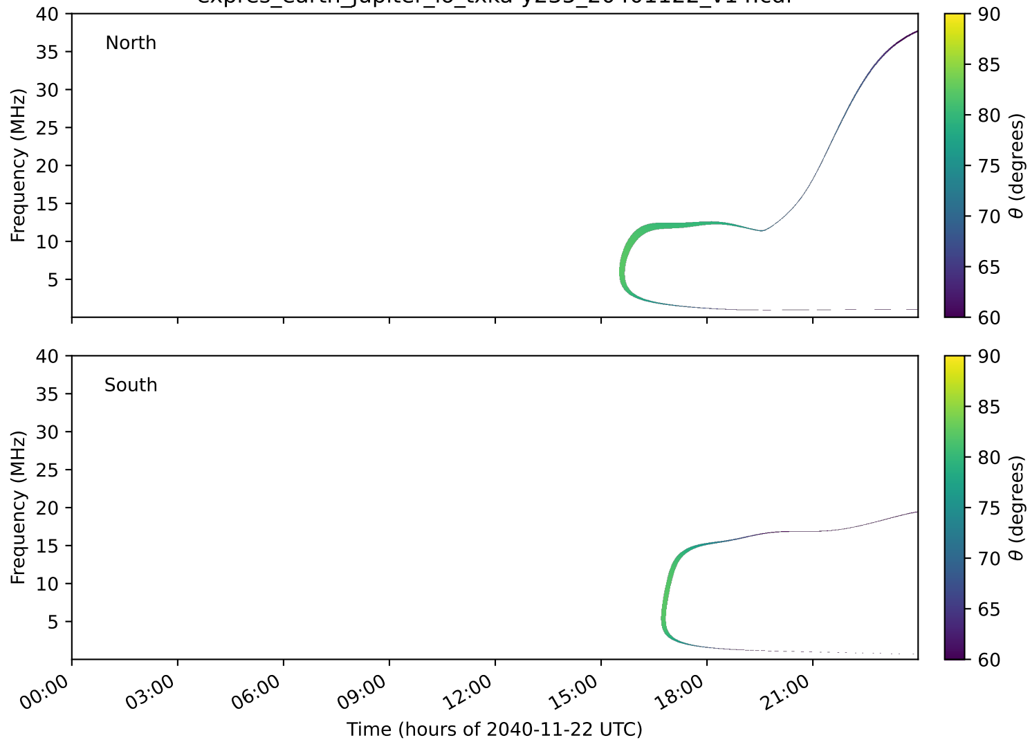
expres_earth_jupiter_io_txka-y235_20401122_v14.cdf
