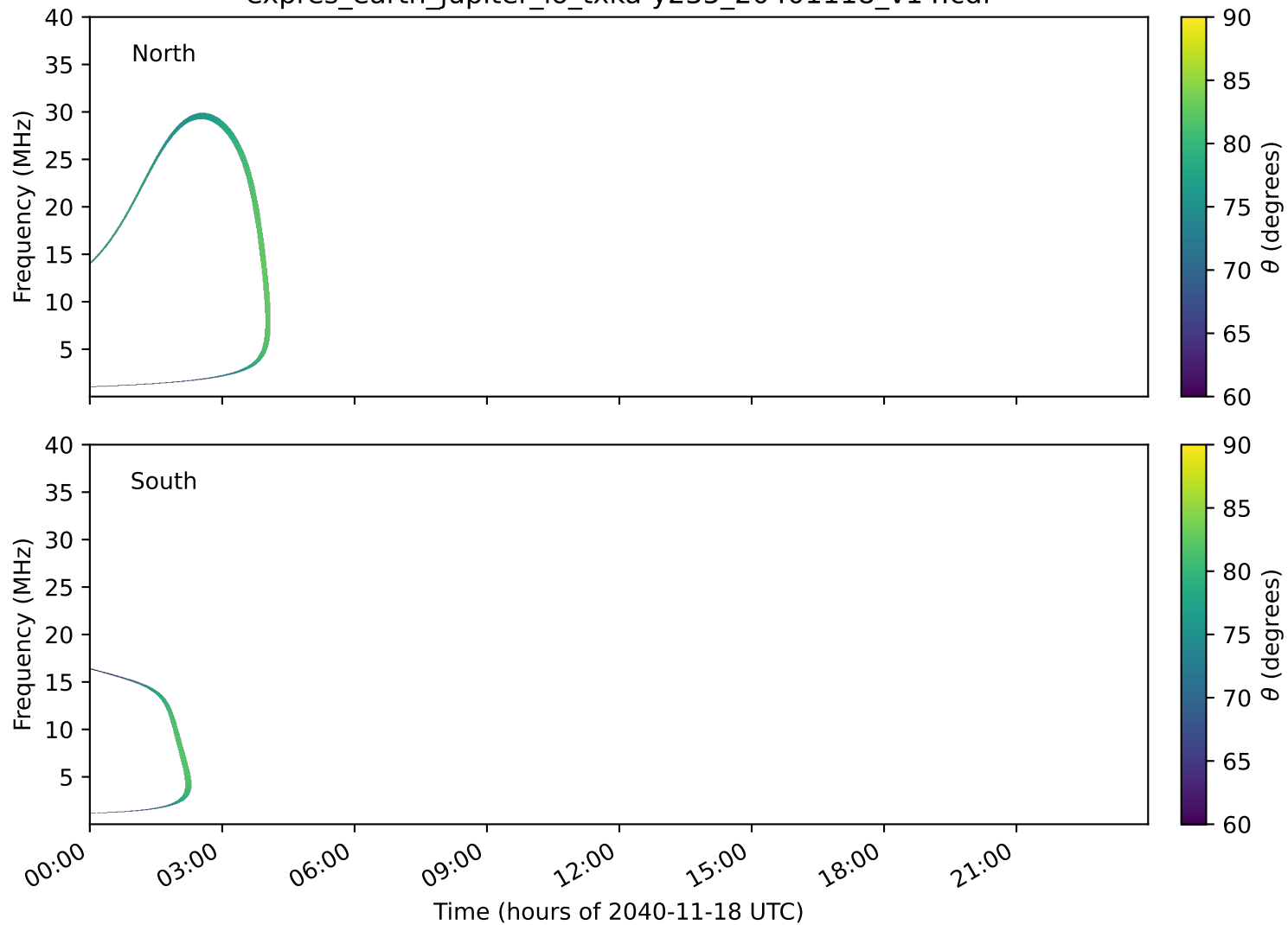
expres_earth_jupiter_io_txka-y235_20401118_v14.cdf
