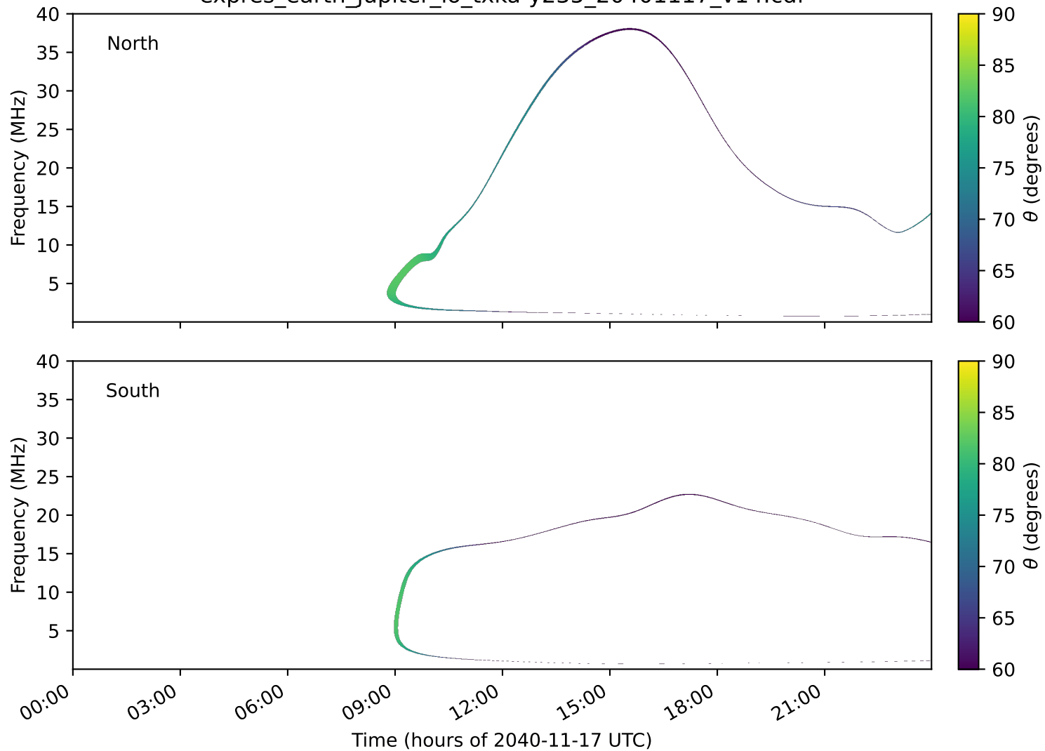
expres_earth_jupiter_io_txka-y235_20401117_v14.cdf
