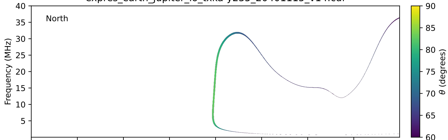
expres_earth_jupiter_io_txka-y235_20401115_v14.cdf
